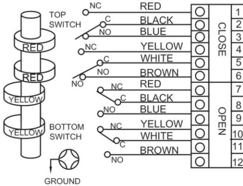
Mechanical Switch (4SPDT) DS300/APL314/ITS300
