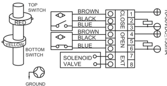
Proximity Switch (3-Wires )PNP NC APL210/DS100/DS300/DS410/DS500
