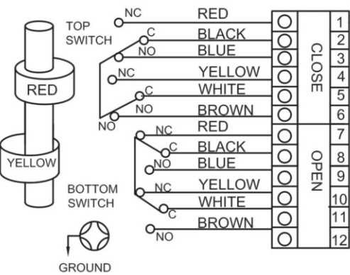
Mechanical Switch (2DPDT) DS300
