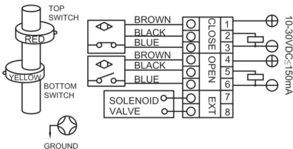
Proximity Switch (3-Wires )PNP NO APL210/DS100/DS300/DS410/DS500
