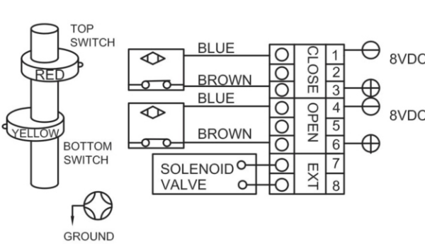
Proximity Switch(2-Wire ) APL220/DS120/DS320/DS420/DS520
