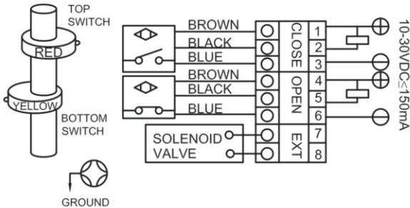
Proximity Switch (3-Wire )NPN NC APL210/DS100/DS300/DS410/DS500
