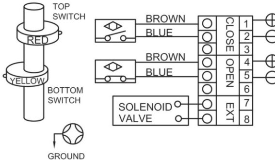
Proximity Switch (2-Wire )NC APL210/DS100/DS300/DS410/DS500
