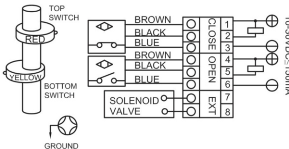
Proximity Switch (3-Wire )NPN NO APL210/DS100/DS300/DS410/DS500
