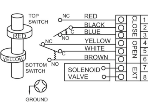
Mechanical Switch (2SPDT) APL210/ITS100/DS100/APL310/DS300/DS410/DS510
